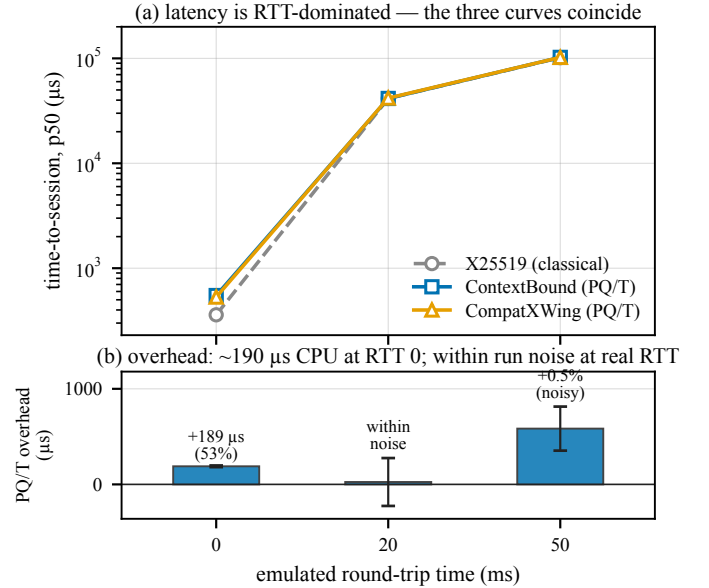
Fig. 6. Historical predecessor-source time-to-session under real tc netem on the virtualized host (mean of two repetitions); the quiesced bare-metal numbers of Table VI supersede it quantitatively, and this figure is retained for the qualitative shape. (a) latency is RTT-dominated—the three curves coincide. (b) the overhead is the fixed local KEX-path overhead at RTT 0 ( \sim 190 \mu\text{s} on this virtualized host; \approx 88 \mu\text{s} on bare metal, Table VI); at realistic RTT it is within run-to-run noise (error bars span the two repetitions and cross zero at RTT 20 ms).
