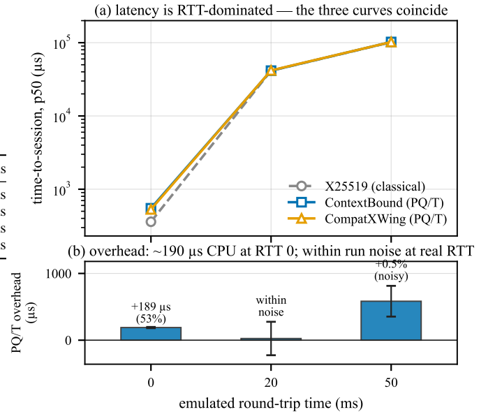
Fig. 6. Time-to-session under real tc netem on the virtualized host (mean of two repetitions); the quiesced bare-metal numbers of Table VI supersede it quantitatively, and this figure is retained for the qualitative shape. (a) latency is RTT-dominated—the three curves coincide. (b) the overhead is the fixed ML-KEM CPU cost at RTT 0 ( \sim 190 \mu\text{s} on this virtualized host; \approx 88 \mu\text{s} on bare metal, Table VI); at realistic RTT it is within run-to-run noise (error bars span the two repetitions and cross zero at RTT 20 ms).
