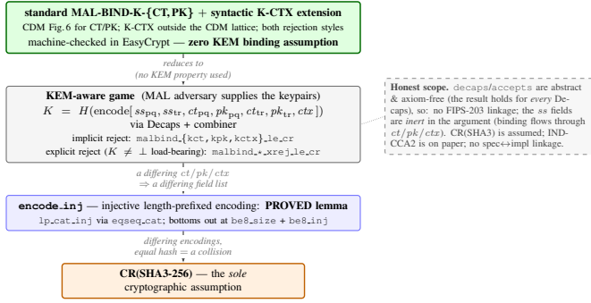
Fig. 2. The kernel as a reduction tower: standard MAL-BIND-K- \{CT,PK\} plus the separately labeled syntactic K-CTX extension (both rejection styles) reduce—using no property of Decaps—through the proved encode_inj to collision-resistance of SHA3, the sole cryptographic assumption.
