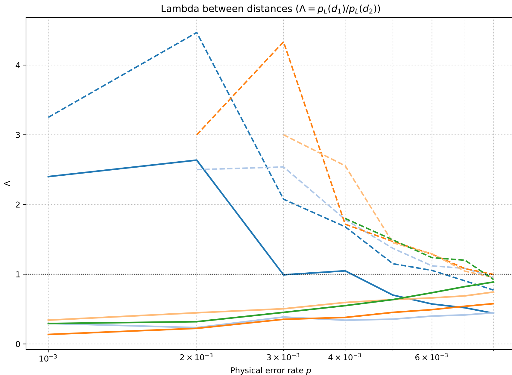
Figure A10. Error suppression factor \Lambda between adjacent distances for GraphSAGE (solid) and MWPM (dashed). Values below 1 indicate improved suppression with distance; the dotted line marks \Lambda = 1 .
