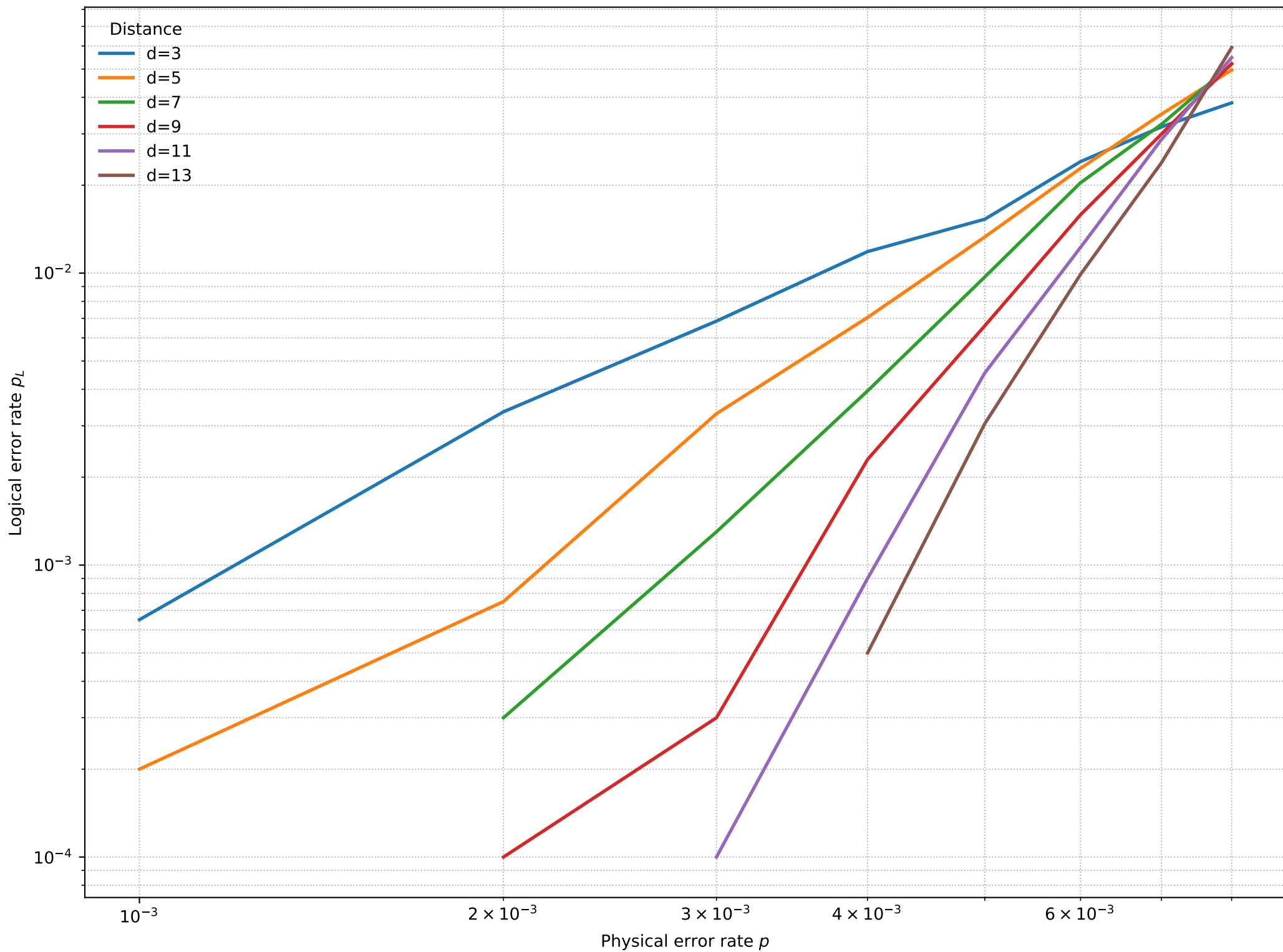
MWPM
