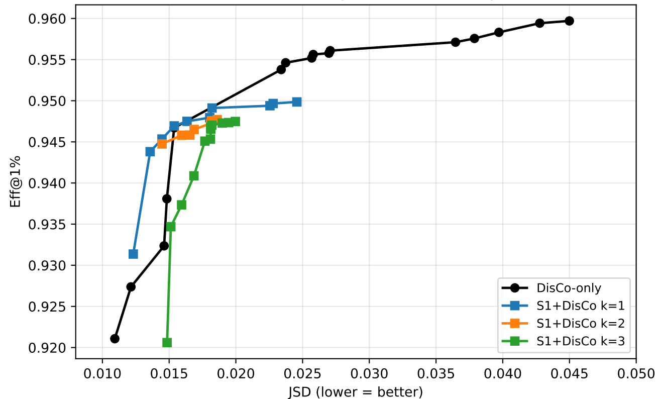
Pareto frontier comparison (Phase 4 ep40)
