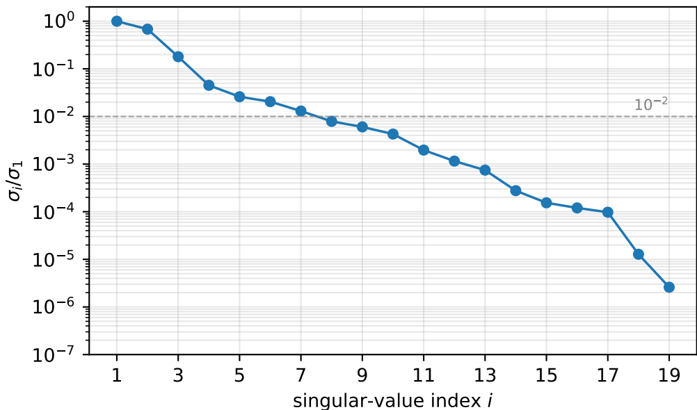
Scree plot of M (QCD class-conditional bin means, B = 20 )
