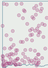
Layer in metres EPSG:32749
