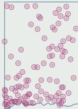
Layer in metres EPSG:32749
