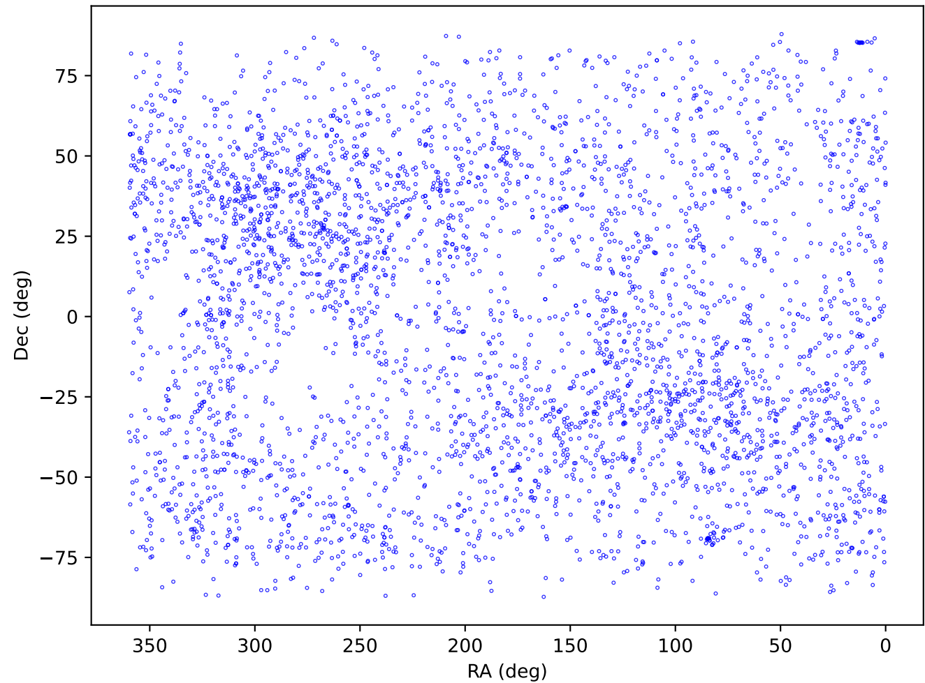
Catalog sources (RA / Dec)
