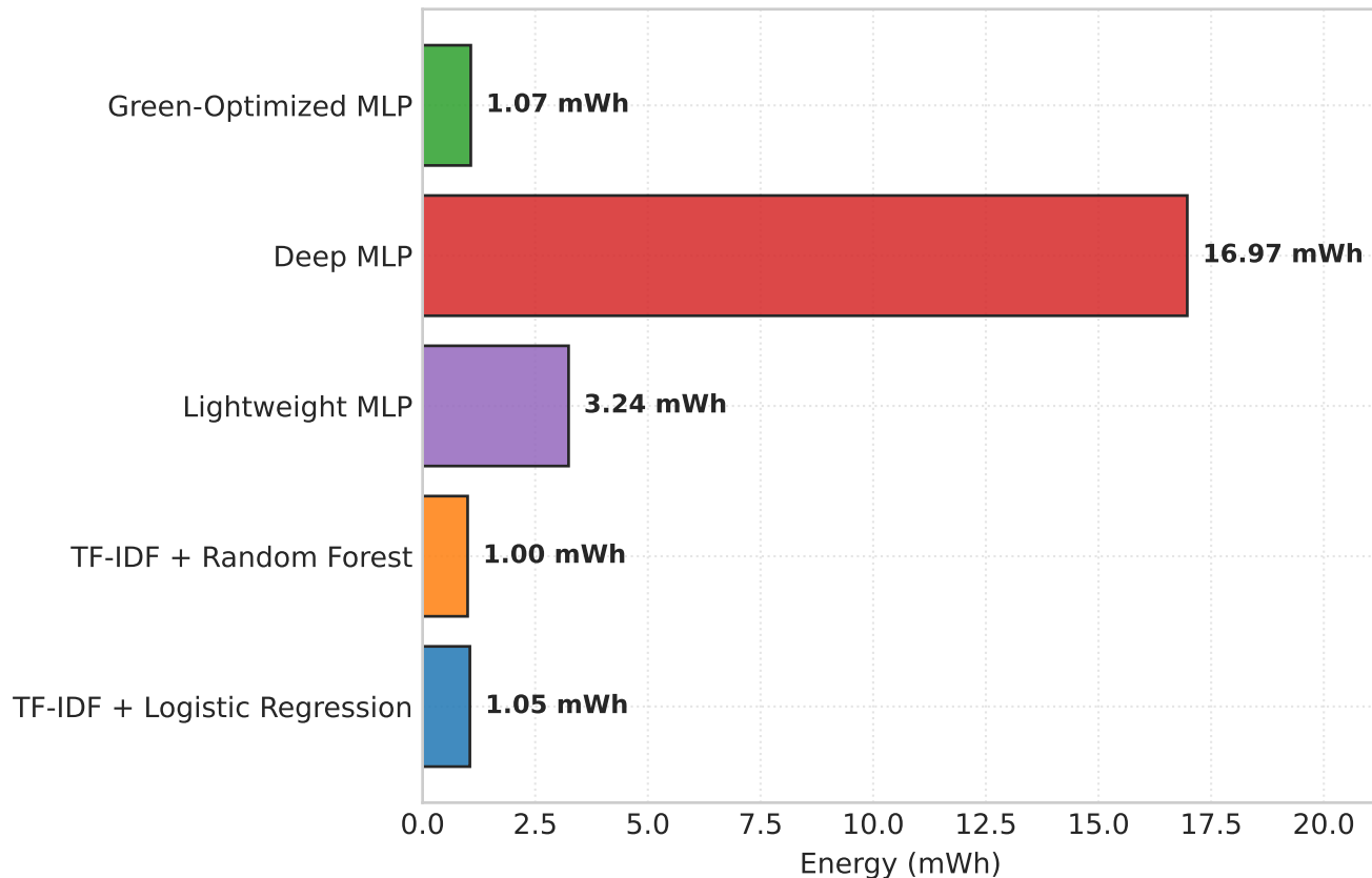
Energy Consumption per Training Run (mWh)
