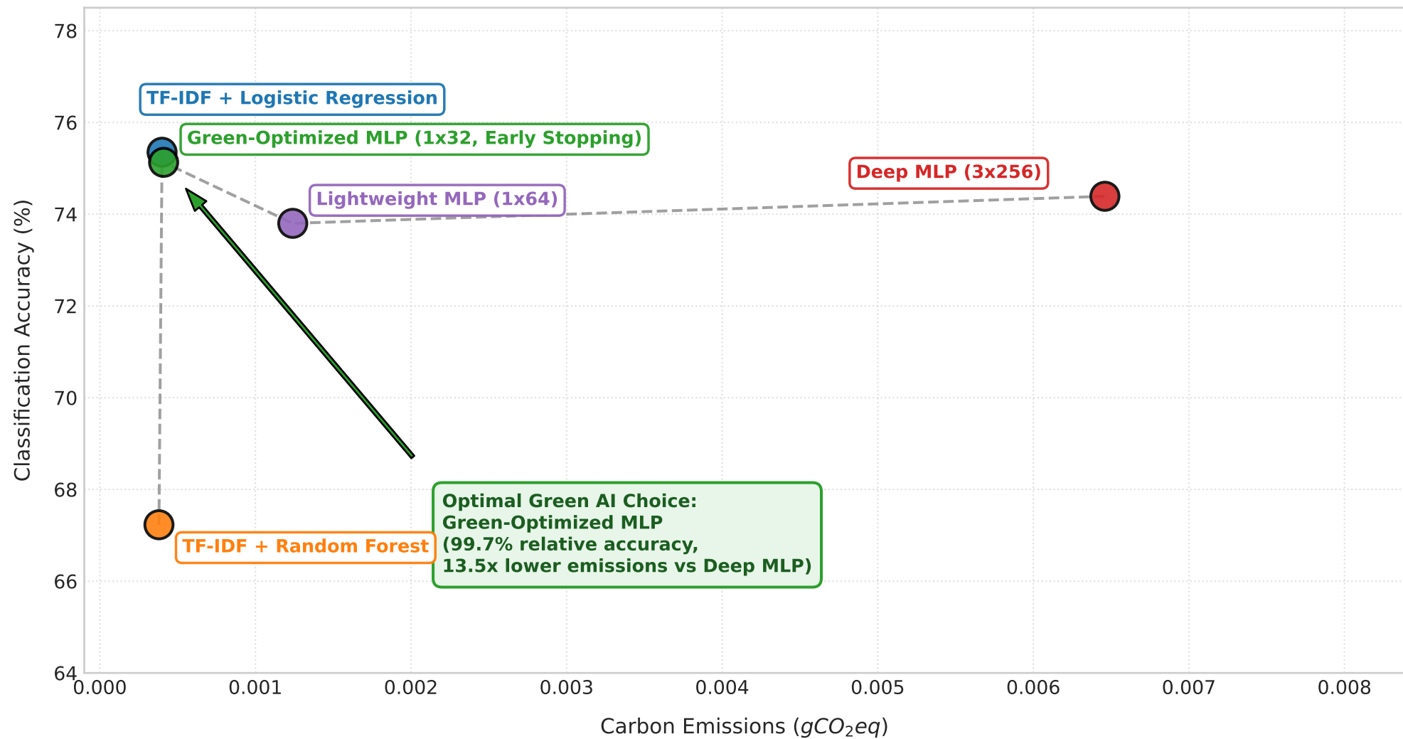
Green AI Pareto Frontier: Accuracy vs. Carbon Emissions ( gCO_2eq )
