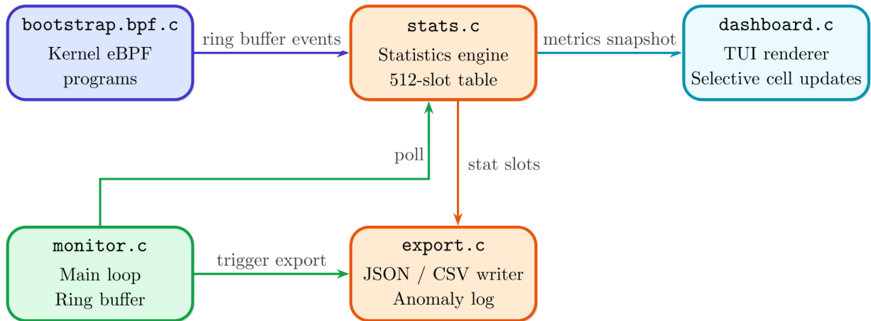
Figure 3: Module Dependency
