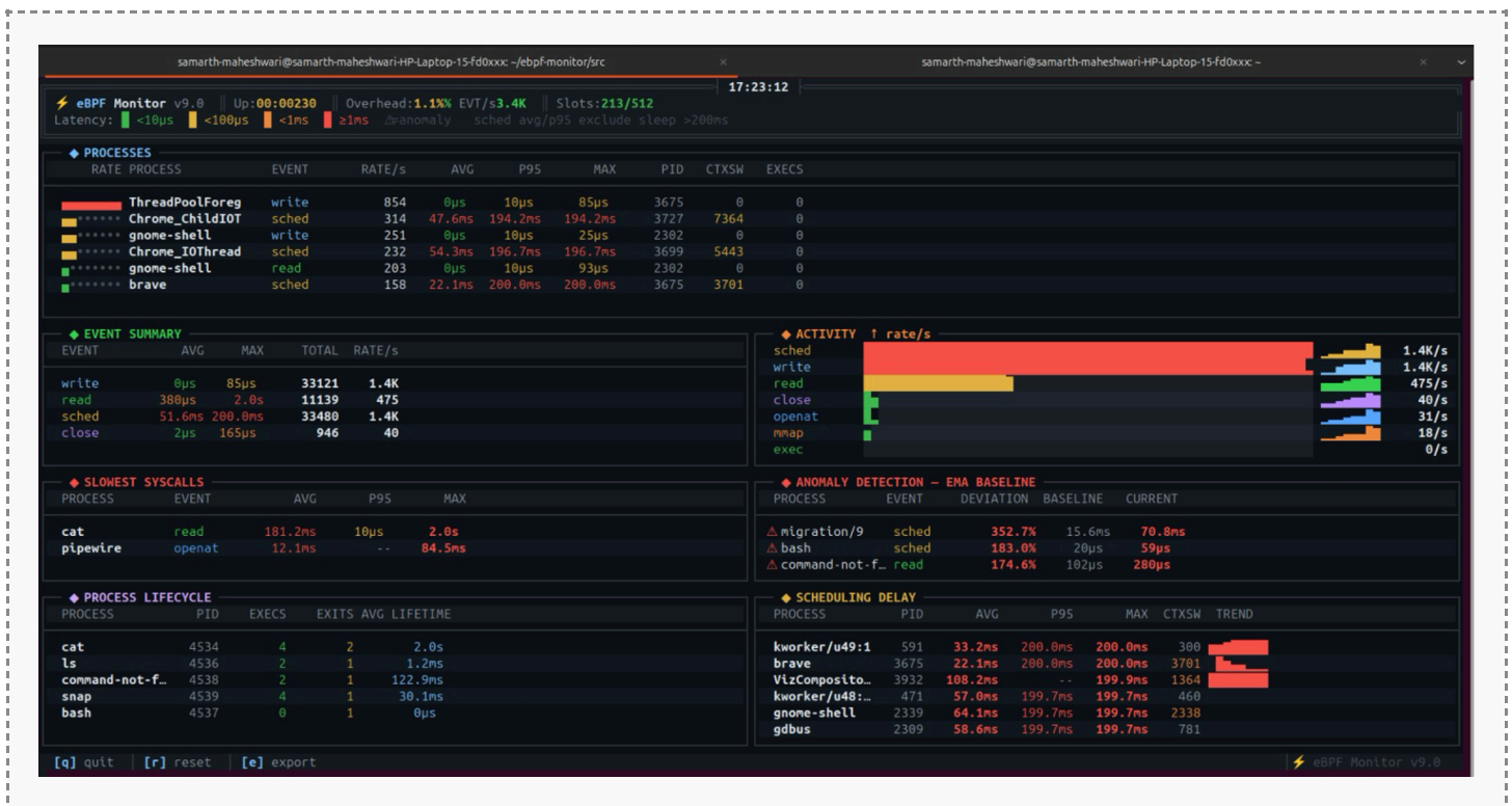
Figure 4: Dashboard Layout
