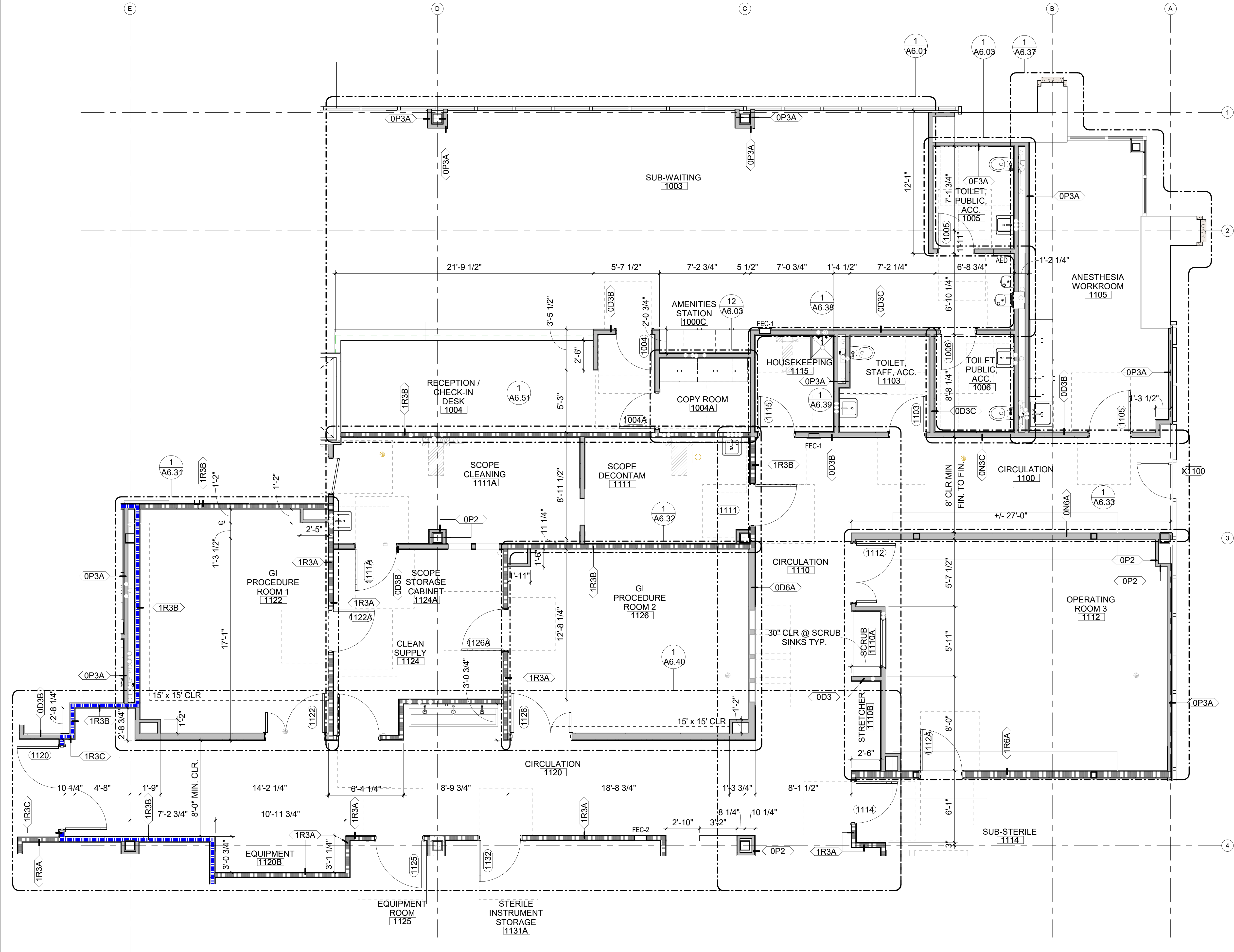
1 ENLARGED FLOOR PLAN LEVEL 1 - AREA B 1/4" = 1'-0"
