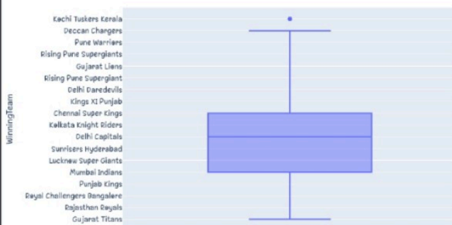
Box Plot
