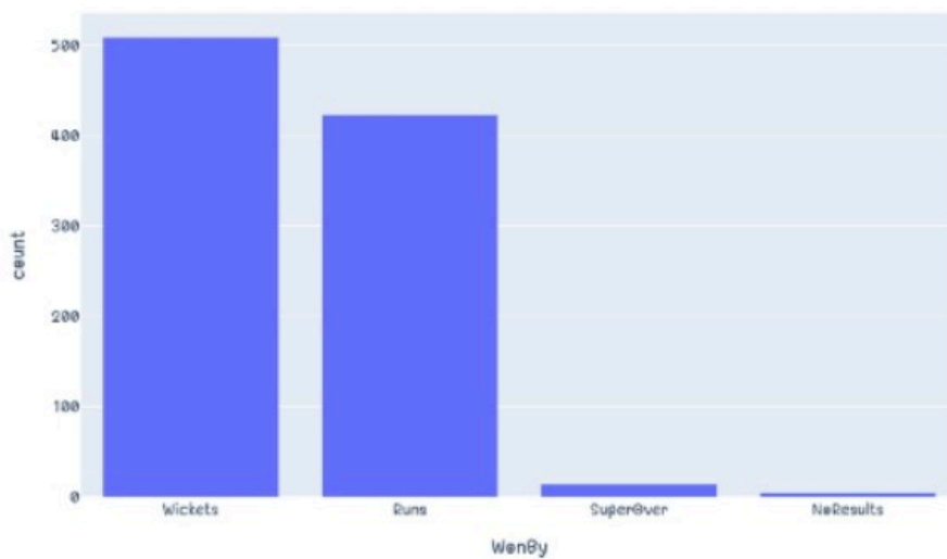
Histogram
