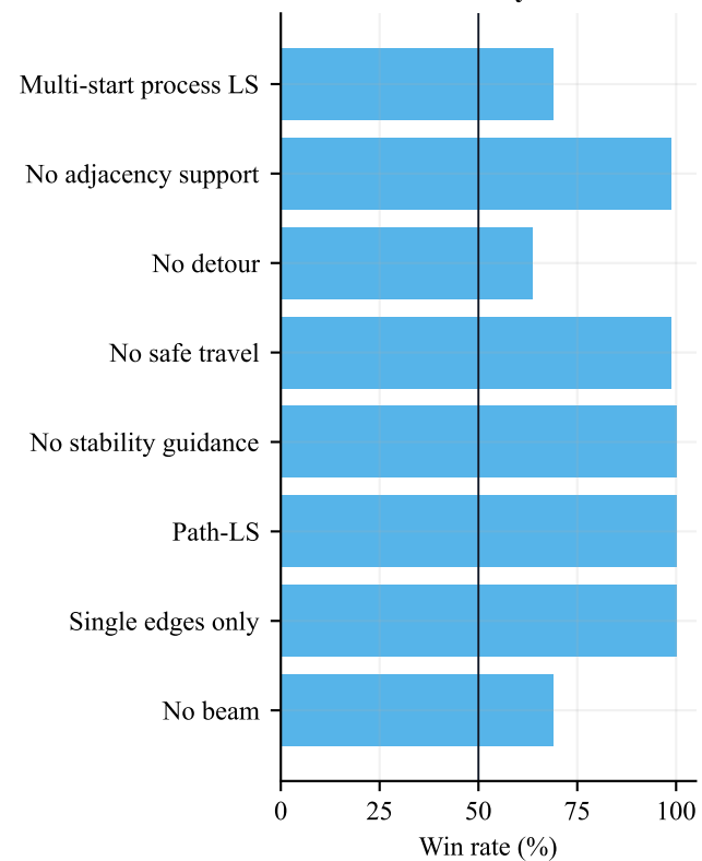
Process-key wins
