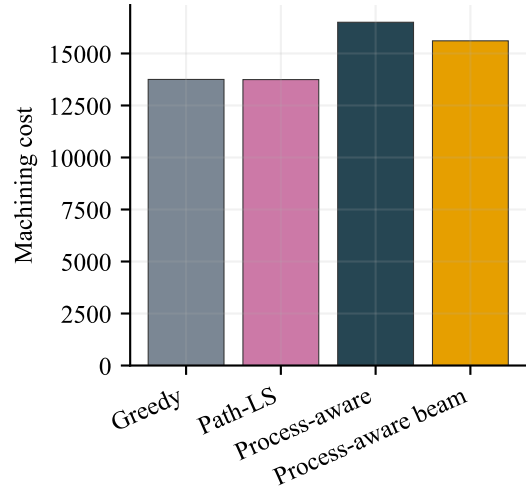
Machining cost
