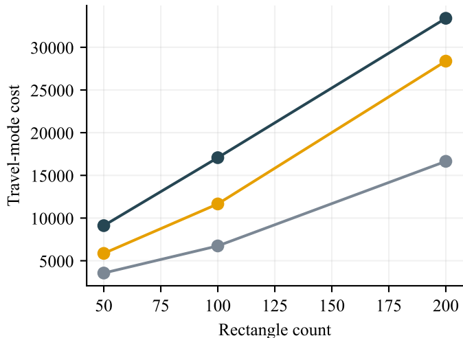
Cost scaling
