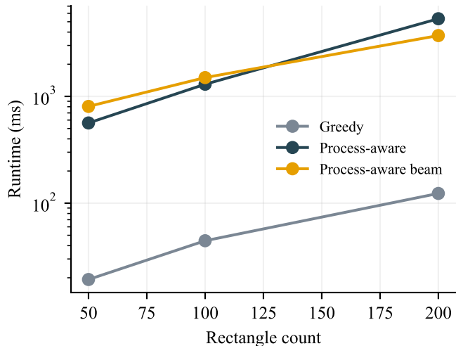
Runtime scaling
