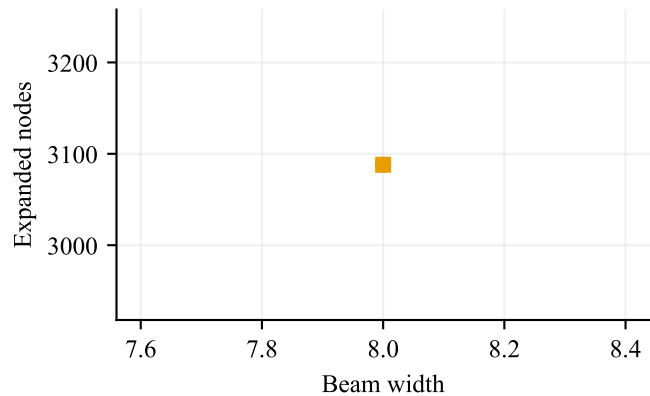
Expanded nodes
