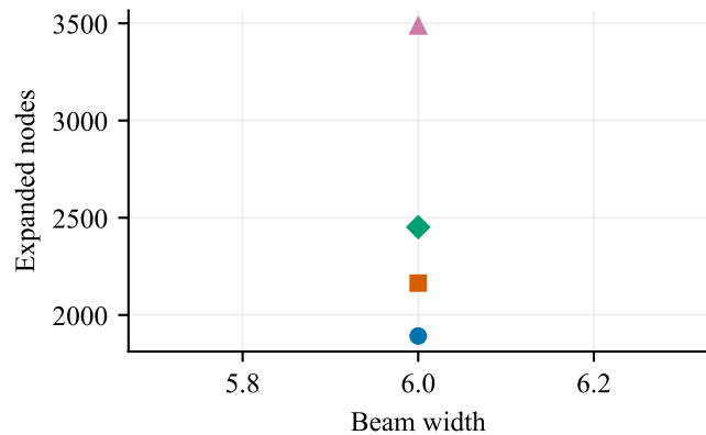
Expanded nodes
