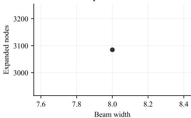
Expanded nodes
