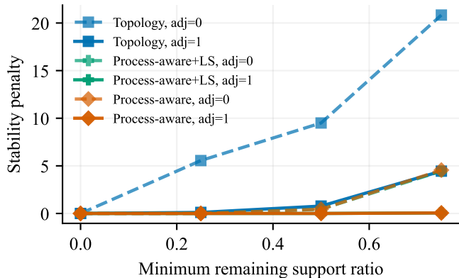
Stability penalty
