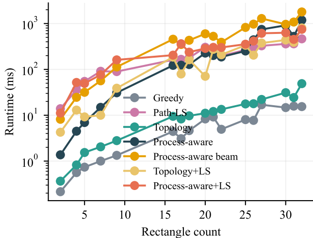
Runtime scaling
