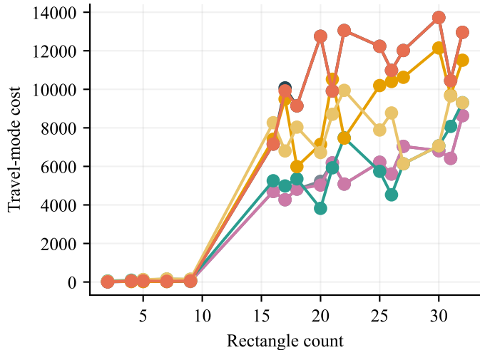
Cost scaling
