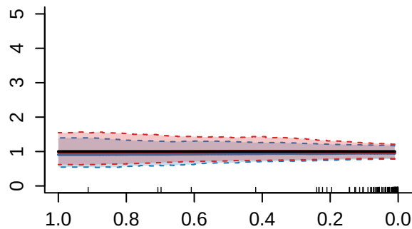
Discrete (phylodyn)
