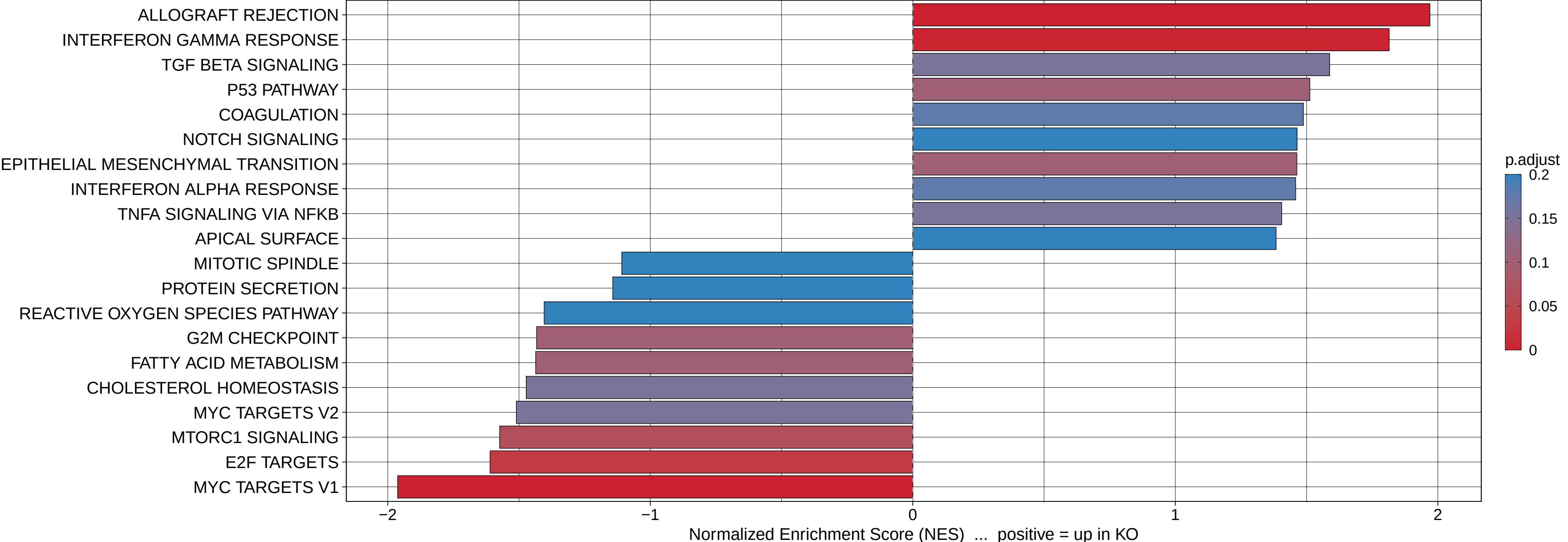
GSEA ... Hallmark (H) top 10 pathways per direction, sorted by NES; fill = p.adjust (0...0.2)
