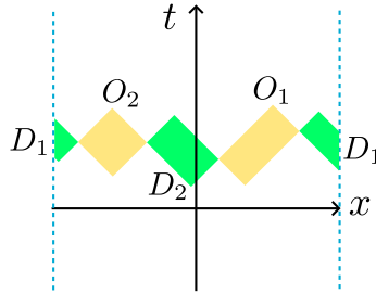
Figure 2.3. The causal complement D_1 \cup D_2 of O_1 \cup O_2 , projected onto \mathbb{R}_{(-\pi, \pi)}^{1,1}
