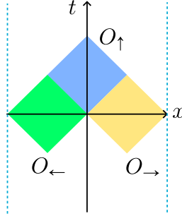
Figure 2.2. The double cones O_{\uparrow}, O_{\rightarrow}, O_{\leftarrow} in \mathbb{R}_{(-\pi, \pi)}^{1,1}
