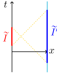
Figure 3.1. Boundary-boundary Haag duality in \mathbb{R}_{\text{op}}^{1,1}
