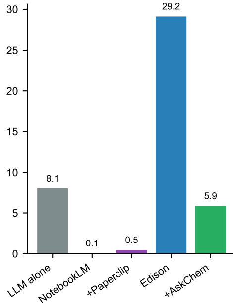
Grounded specificity
