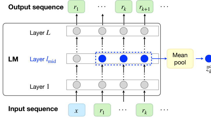
Figure 2: LM-based anchor construction for ReasonFlow. As one concrete instantiation of ReasonFlow, we construct reasoning anchors using a causal transformer language model. The LM reads the sequence (x, r_1, \dots, r_K, y) . For each step k , we mean-pool the middle-layer hidden states over the prefix up to r_k , then project and sphere-normalize the result to obtain anchor z_k^a . This LM-based construction is one concrete instantiation of ReasonFlow while the framework itself only requires a sequence of continuous reasoning anchors.
