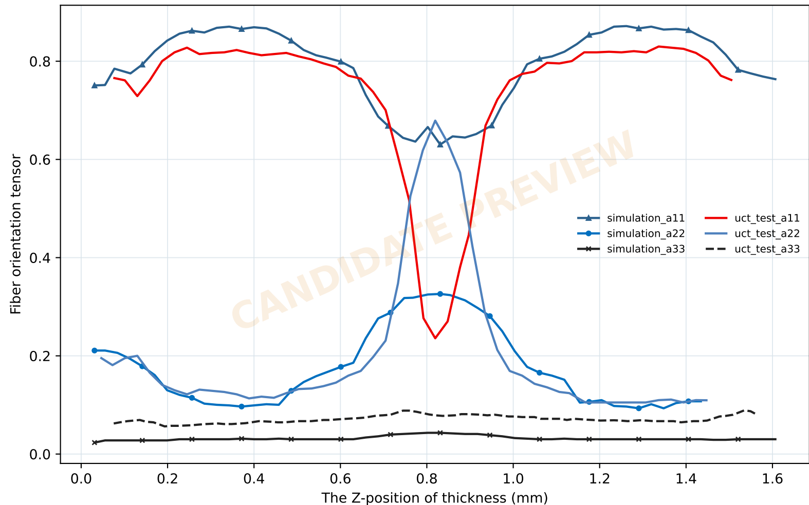
Fig. 9 Fiber orientation tensors CANDIDATE PREVIEW — NOT HUMAN-REVIEWED
