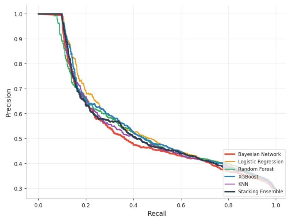
Precision-Recall Curves — All Models
