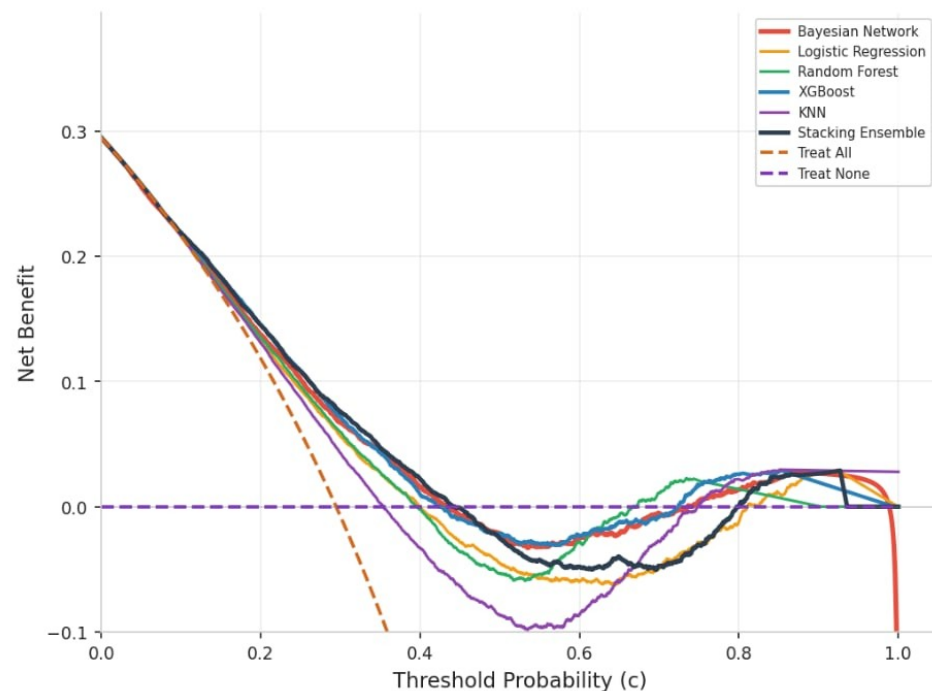
Decision Curve Analysis — All Models
