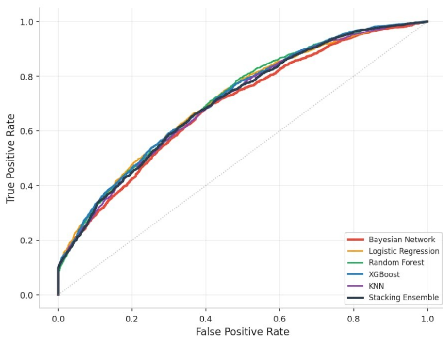
ROC Curves — All Models
