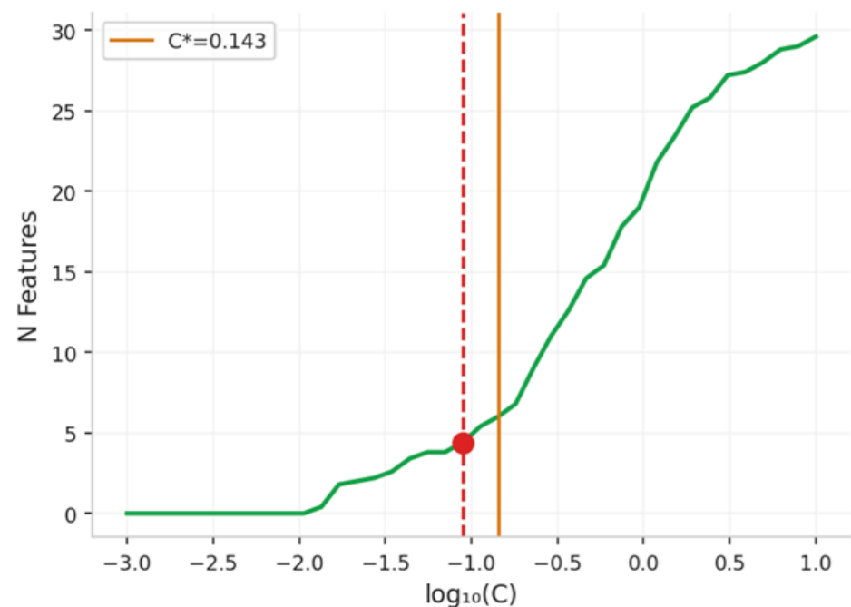
② N Features Selected (Elbow)
