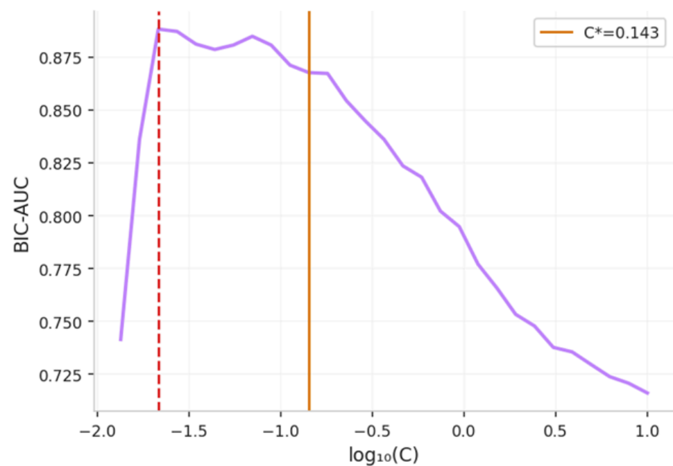
③ BIC-penalized AUC
