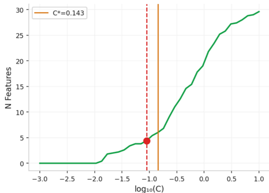
② N Features Selected (Elbow)
