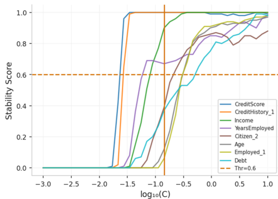
④ Stability Selection Path
