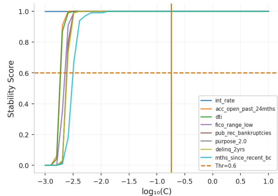
④ Stability Selection Path
