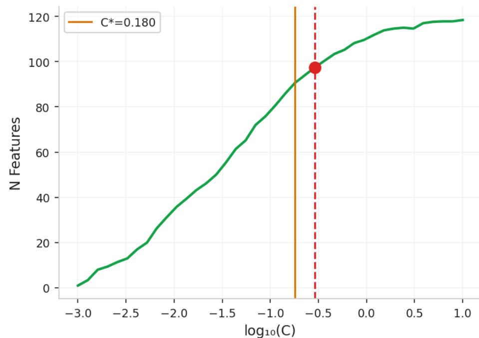
② N Features Selected (Elbow)
