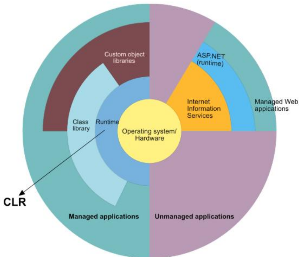
Role of CLR in the execution of a C# program
