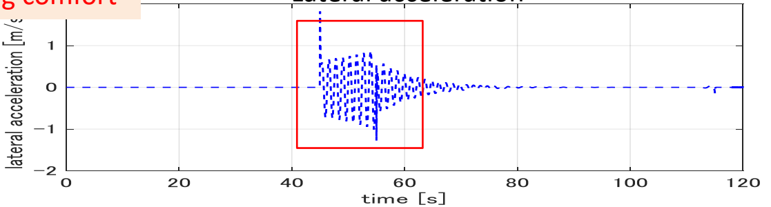
Lateral acceleration
