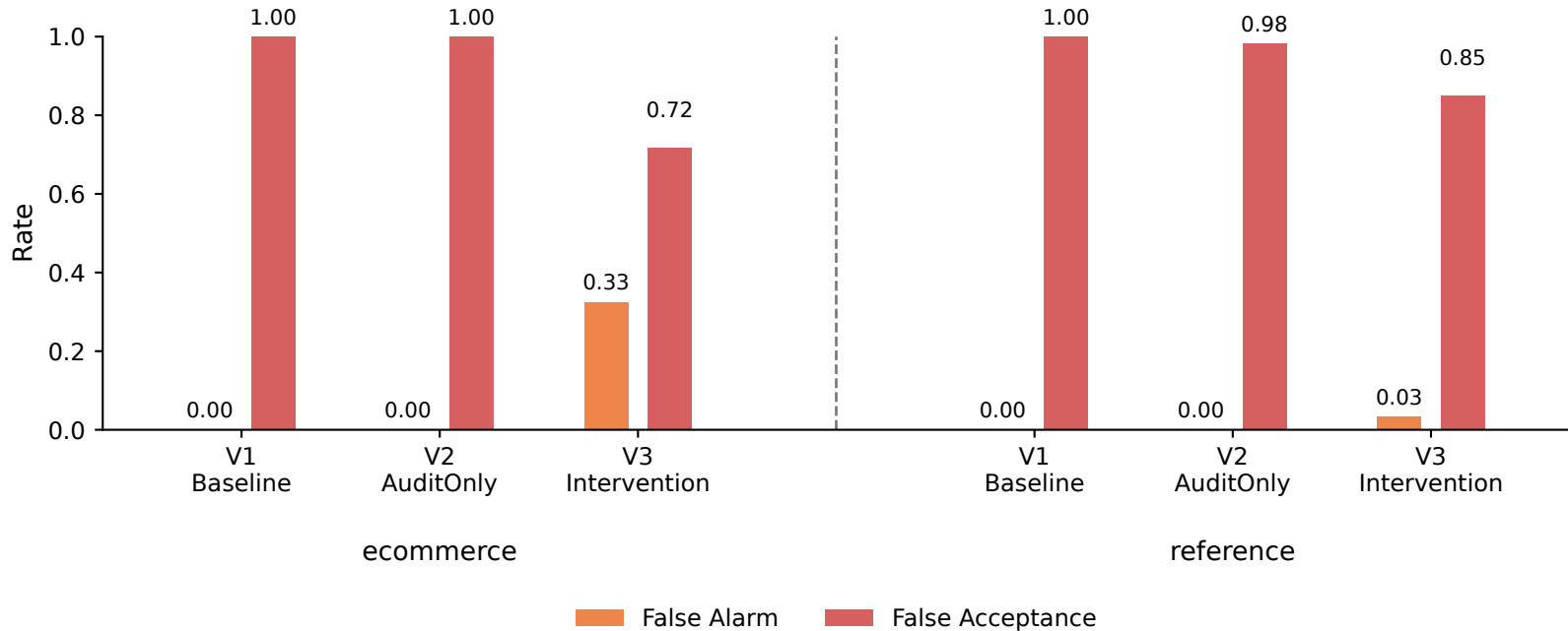
Set B: Generalization Test
