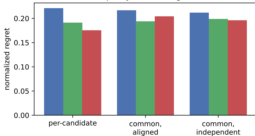
7-policy slate — regret
