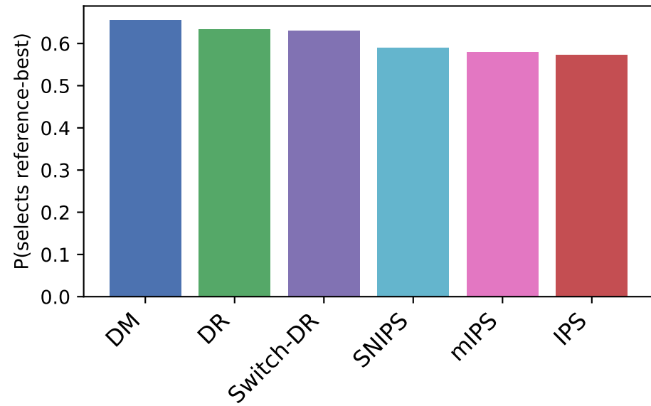
(a) Reference-best selection rate
