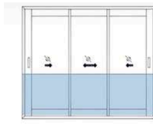
3T + 3G Shutter, Sliding Window
