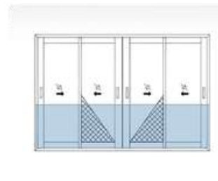
3T + 4G Shutter, Sliding 2 Mesh Shutter Sliding Window
