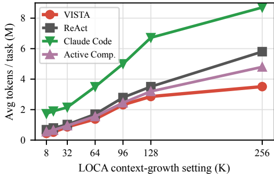
(b) Token cost vs. context-growth setting
