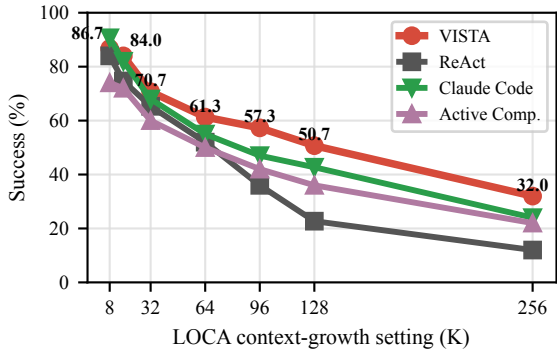
(a) Success vs. context-growth setting
