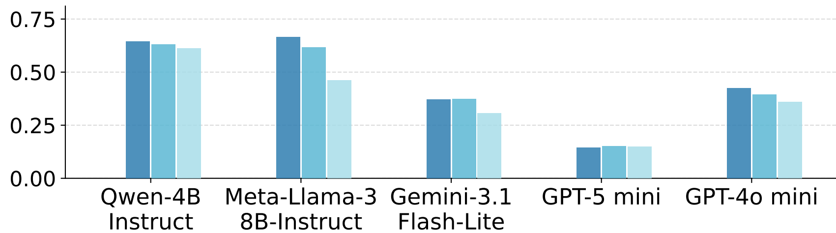
Empirical ECE (Answered)
