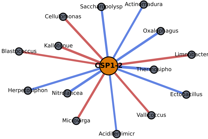
(b) Deep — CSP1-2 ego network (14 co-occurring genera)
