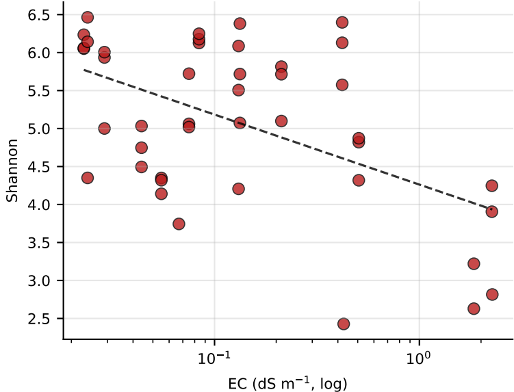
(h) Atacama — salinity suppresses diversity \rho = -0.38 , p = 0.012
