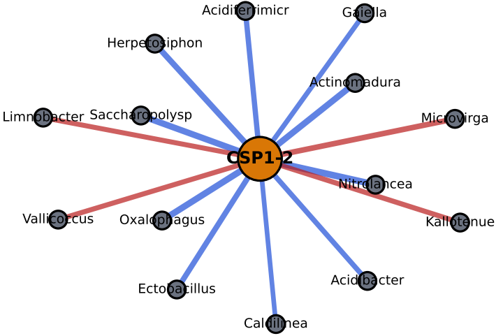
(a) Surface — CSP1-2 ego network (14 co-occurring genera)
