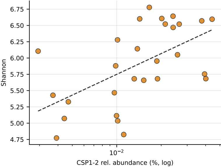
(g) Namib — abundance tracks diversity \rho = +0.64 , p = 1.4 \times 10^{-4}
