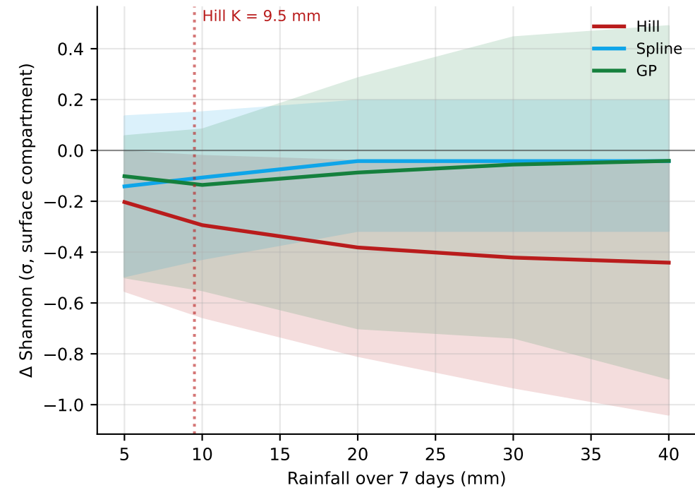
(b) Non-linear rainfall dose-response (Hill / spline / GP)
