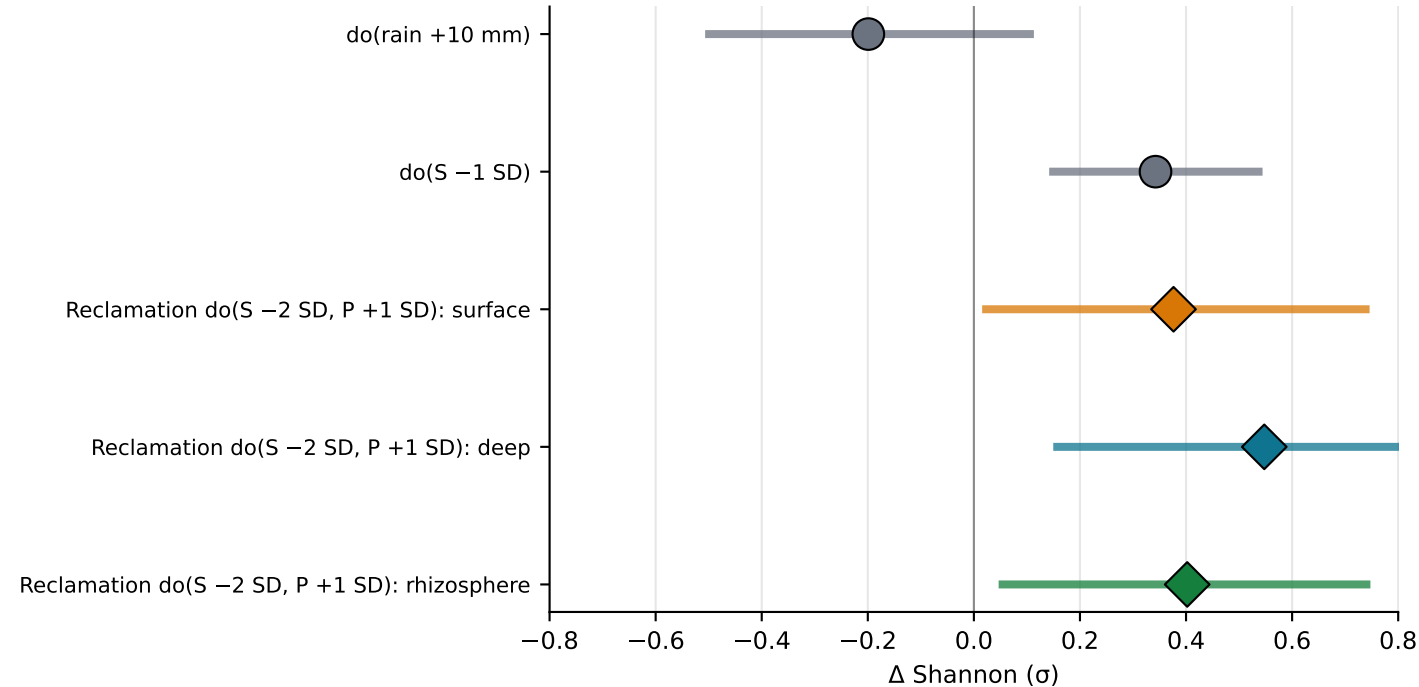
(c) Interventional posteriors (Bayesian state-space digital twin)
