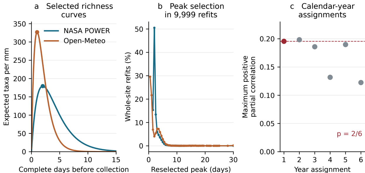
Figure S1: Rainfall associations, refitted timing distributions and complete calendar-year search. (a) Selected richness kernels for NASA POWER and Open-Meteo, expressed as expected taxa per millimetre of antecedent rain. Points mark the fitted peaks. (b) Richness-peak selection frequencies across 9,999 whole-site samples, with every nuisance model refitted. (c) The joint maximum positive partial correlation across both products, all 60 peaks and all 3 endpoints for each of the six year assignments listed in Table S11. Red marks the observed assignment, which ranked second ( p = 2/6 ).
