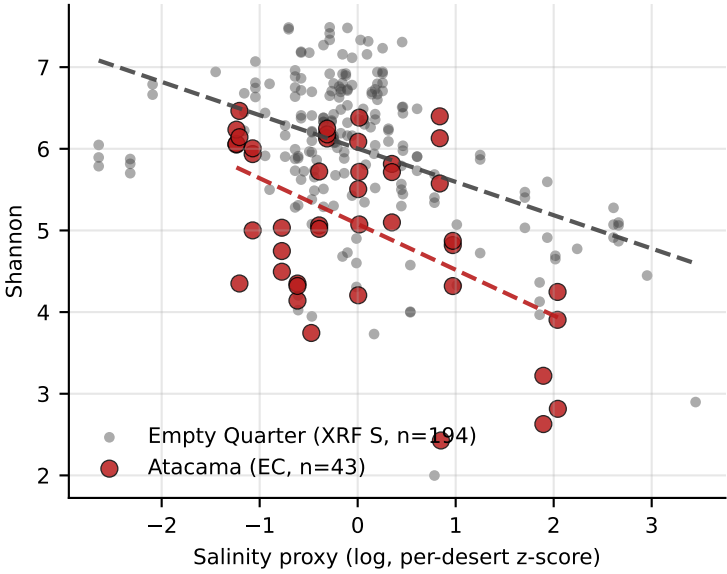
(h) Salinity vs Shannon (EQ + Atacama) EQ (XRF S): \rho=-0.34 , p=1.4e-06 | Atacama (EC): \rho=-0.38 , p=1.2e-02
