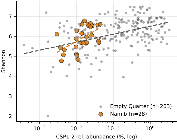
(g) CSP1-2 abundance vs Shannon (EQ + Namib) EQ: \rho=+0.37 , p=4.4e-08 | Namib: \rho=+0.58 , p=1.1e-03
