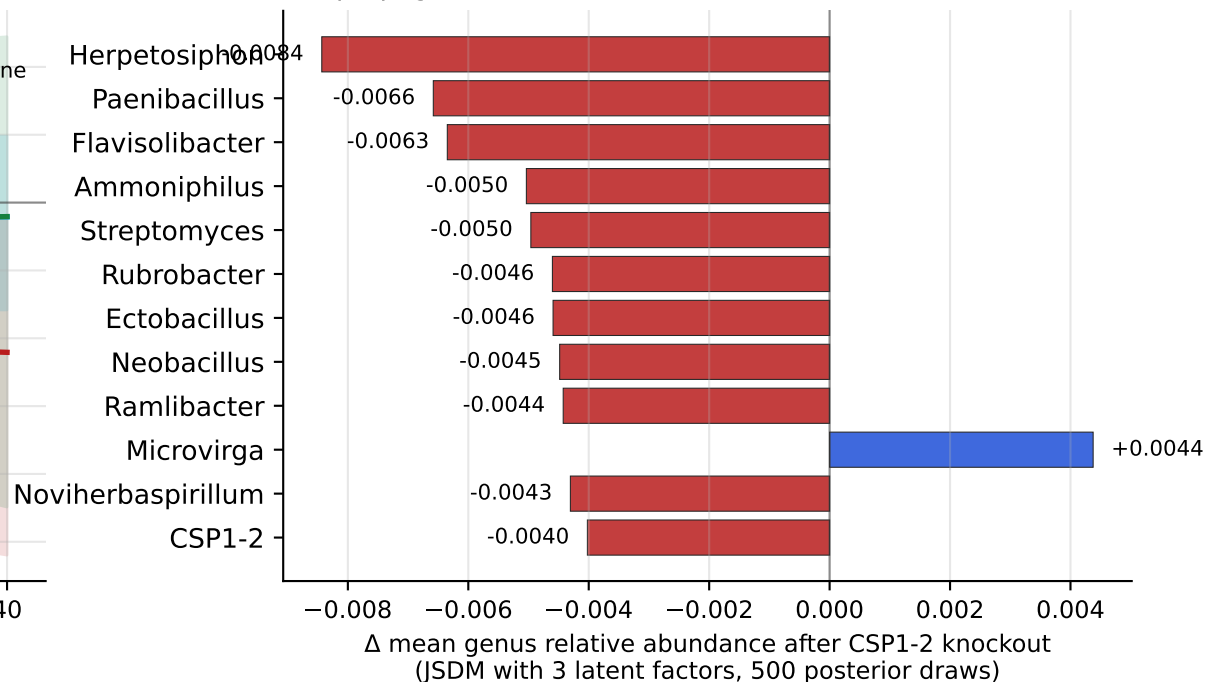
(d) JSDM knockout: top 12 genera affected by CSP1-2 removal (propagates to \Delta Shannon \approx -0.35 via biotic associations)
