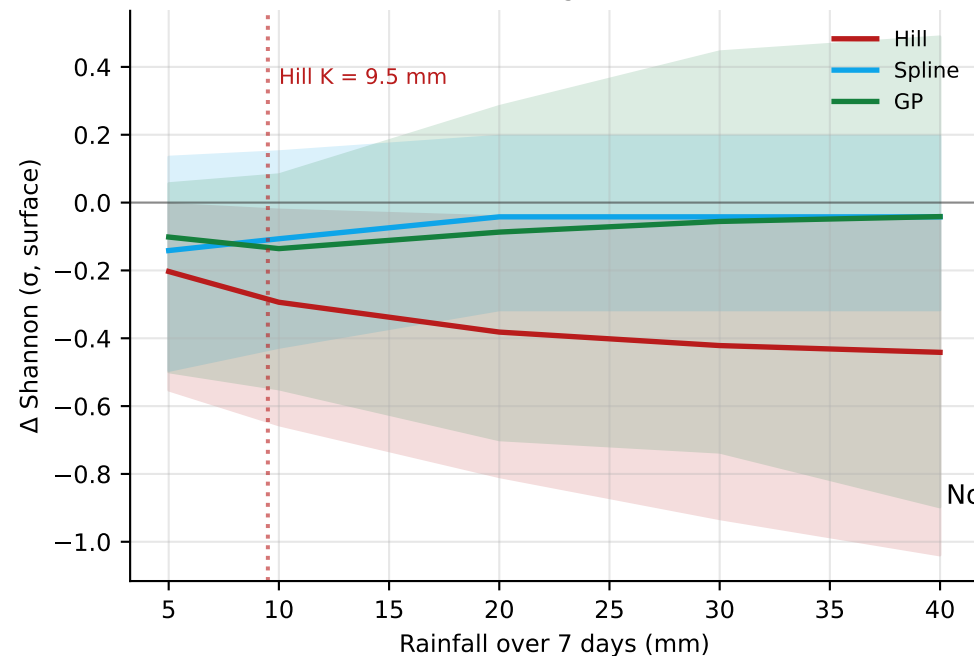
(c) Rainfall dose-response: three functional forms consistent at small mm, diverge at >20 mm
