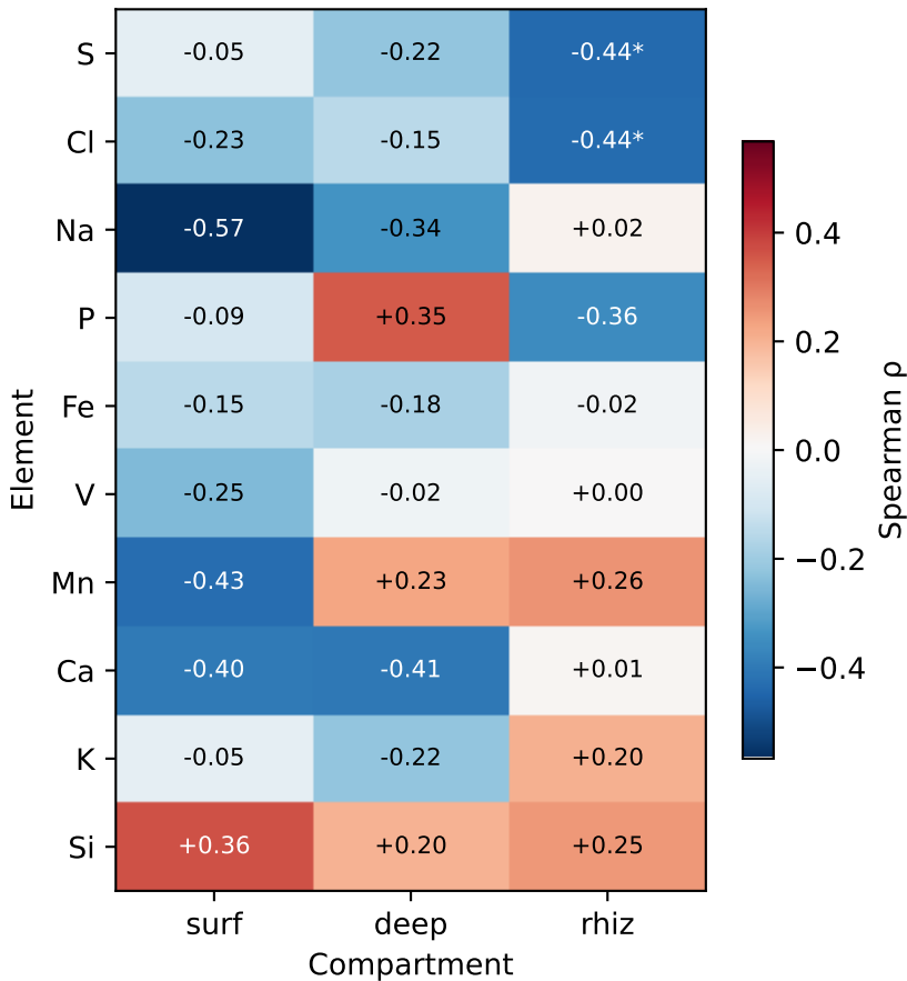
XRF × Shannon (per compartment) Spearman \rho (BH-FDR q < 0.05 marked *)
