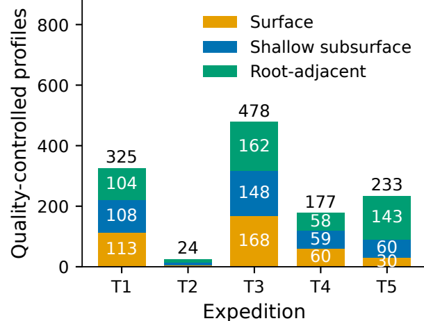
(b) Coverage by compartment
