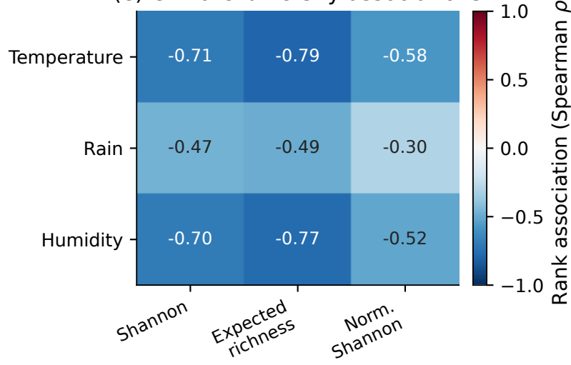
(e) Climate-diversity associations
