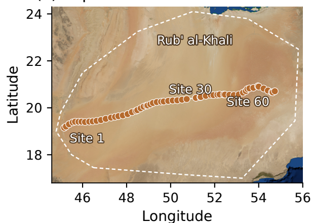
(a) Repeated 60-site desert transect
