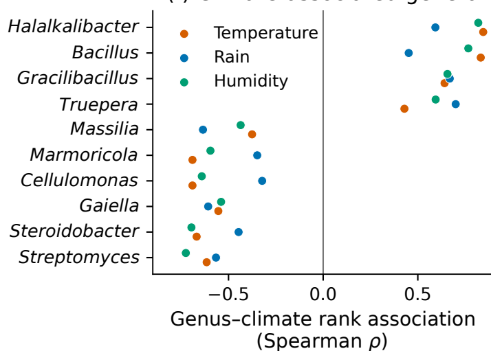
(f) Climate-associated genera
