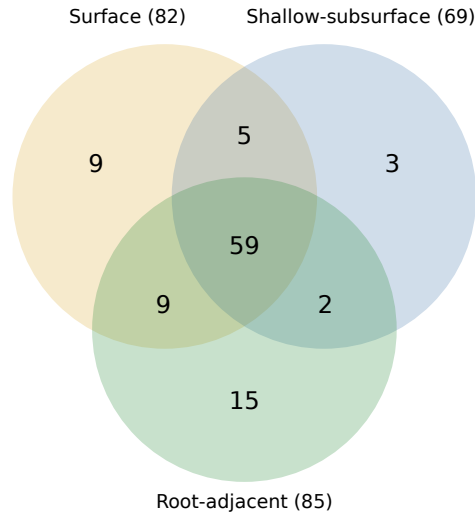
Figure 2. Overlap of core genera among soil compartments. A genus belongs to a compartment's core when it occurs at \geq 90\% of the 60 sites after pooling counts within site and compartment across campaigns and rarefying 20 times to 12,865 reads; detection requires presence in at least half of the draws. Numbers give mutually exclusive intersections; circle areas are schematic.
