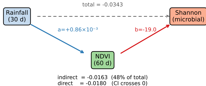
(A) rainfall \rightarrow NDVI \rightarrow Shannon (2k bootstraps)
