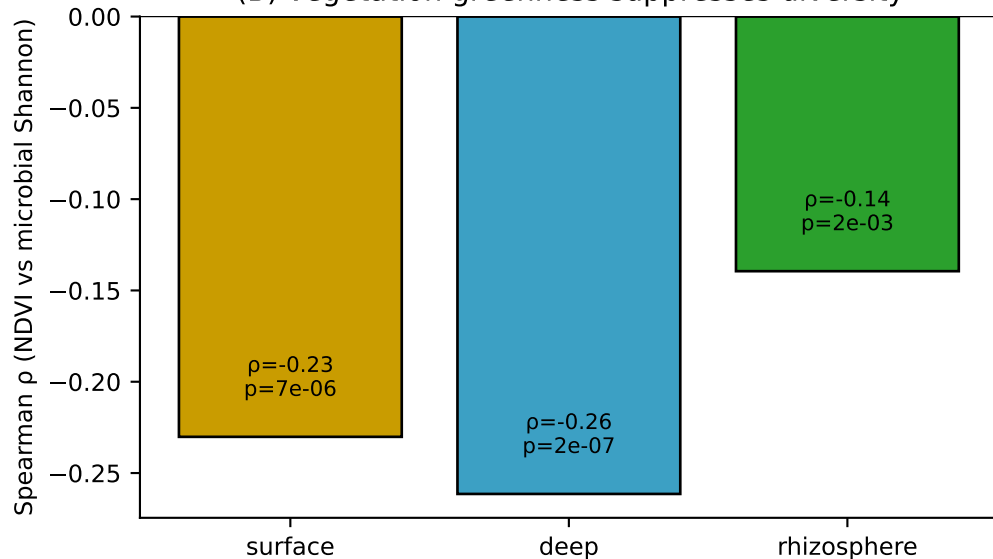
(B) vegetation greenness suppresses diversity
